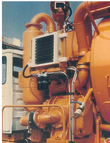
Positive displacement blower Hibon, air injection series, installed on a vacuum truck for sewage cleaning. Installation : FRANCE.
