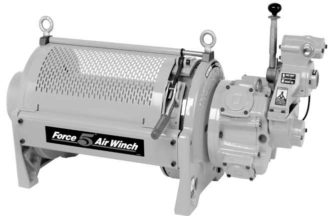
FA2B with manual drum brake, auto disc brake, drum guard, and K5C2 control valve
